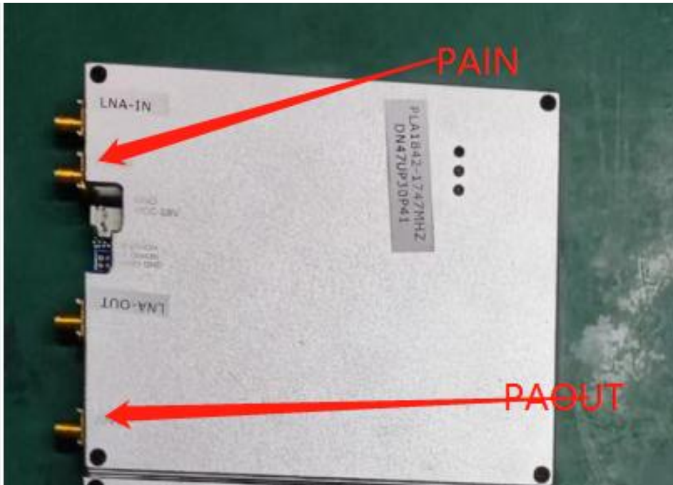
PAIN is the downstream input, PAOUT is the downstream output Downlink input signal is around -8dbm
